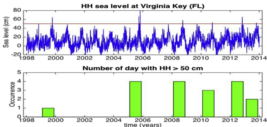
Fig. 4. Tidal and storm flooding events based on the Virginia Key (VK) tide gauge record with threshold of 50 cm above the NAVD datum (horizontal red line) (a). A histogram of flooding occurrence showing a significant increase in annual occurrence after 2006 (b). (For interpretation of the references to color in this figure legend, the reader is referred to the web version of this article.)
